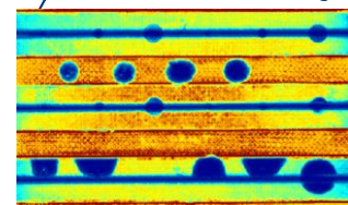
XARION C-scan image
