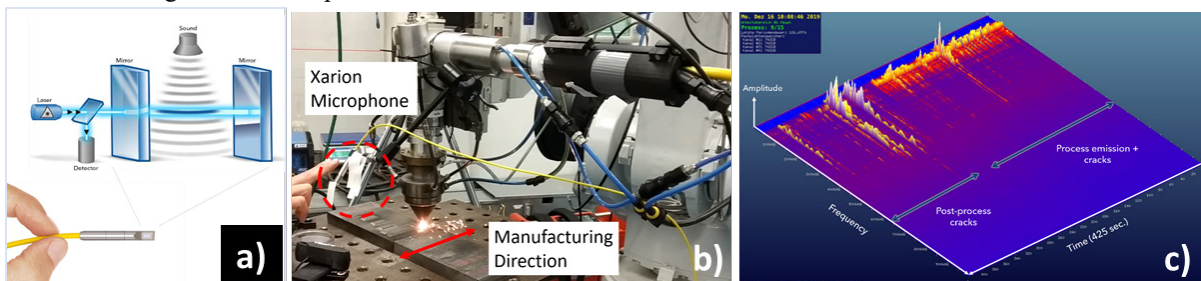
Fig. 1. (a) Optical microphone principle and size (b) LMD manufacturing and in-situ sensing system (c); Spectrogram representation as output from monitoring software containing both process and crack signals.
